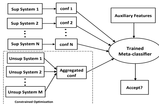
Figure 1: Illustration of our approach to combine supervised and unsupervised ensembles.
