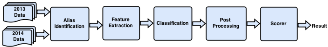
Figure 2: Our system pipeline for evaluating supervised ensembling approaches
