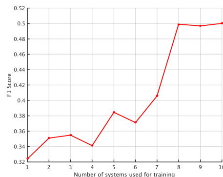
Figure 4: Results for training on 2013 by adding a system at each step and testing on 2014 common systems dataset
